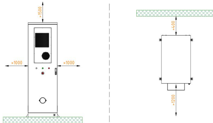
Figure 5-1 Single cabinet
