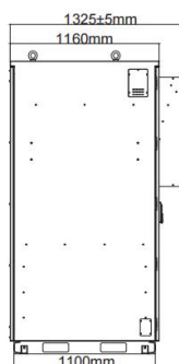
Figure 2-3 Fork position dimensions
