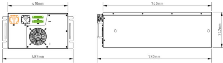
Figure 2-6 Battery Pack appearance and dimensions
