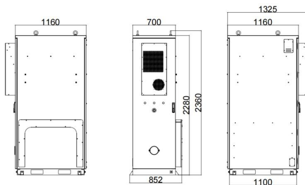
Figure 2-2 Appearance and dimensions
