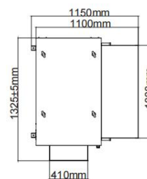
Figure 2-4 Angle supports position dimensions
